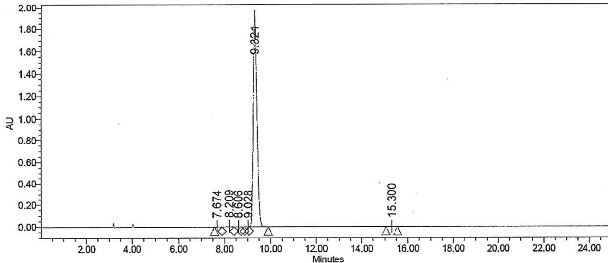
Auto-Scaled Chromatogram
